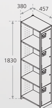
Shelf height = 435
