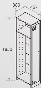
Shelf height = 435 / 1245
