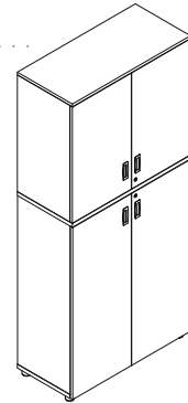
Pre-laminated storage (two door unit) Height - 1986 Width - 750 / 900 Depth - 425
