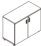
Pre-laminated storage (two door unit) Height - 700 Width - 750 / 900 Depth - 425
