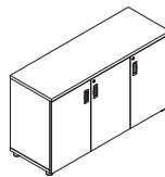
Pre-laminated storage (three door unit) Height - 700 Width - 1050 / 1200 Depth - 425
