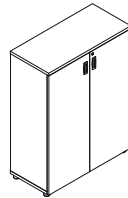
Pre-laminated storage (two door unit) Height - 1200 Width - 750 / 900 Depth - 425
